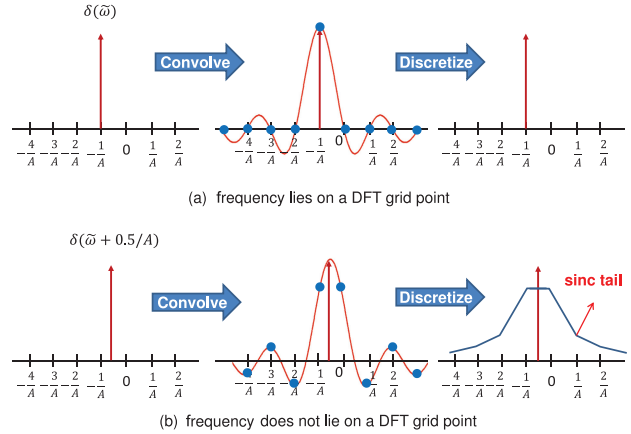
Fig. 2. The windowing effect: limiting samples to an aperture A is equivalent to convolving the spectrum with a sinc function. (a) If a frequency spike lies on a DFT grid point, then the sinc disappears when it is discretized and the original sparsity of the spectrum is preserved; (b) if the frequency spike is not on the DFT grid, once we discretize we get a sinc tail and the spectrum is no longer as sparse as in the continuous domain.
