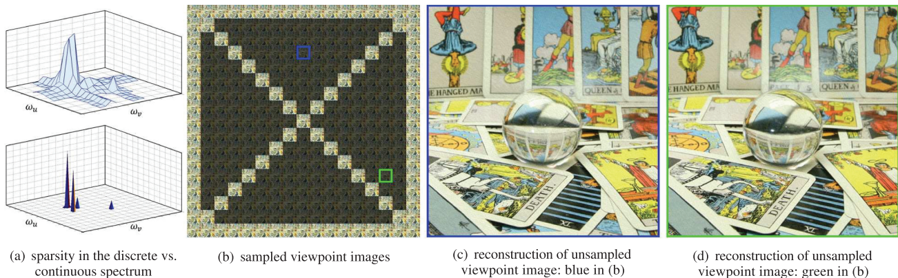
Fig. 1. Sparsity in the discrete vs. continuous Fourier domain, and our reconstruction results: (a) The discrete Fourier transform (top) of a particular 2D angular slice \omega_u, \omega_v of the crystal ball's light field, and its reconstructed continuous version (bottom); (b) a grid showing the original images from the Stanford light field archive. The images used by our algorithm are highlighted (courtesy of Stanford [2008]); (c) and (d) two examples of reconstructed viewpoints showing successful reconstruction of this highly non-Lambertian scene that exhibits caustics, specularities, and nonlinear parallax. The uv locations of (c) and (d) are shown as blue and green boxes in (b).
