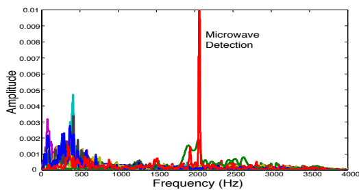
Figure 3. Microwave oven’s acoustic signature on the frequency domain
