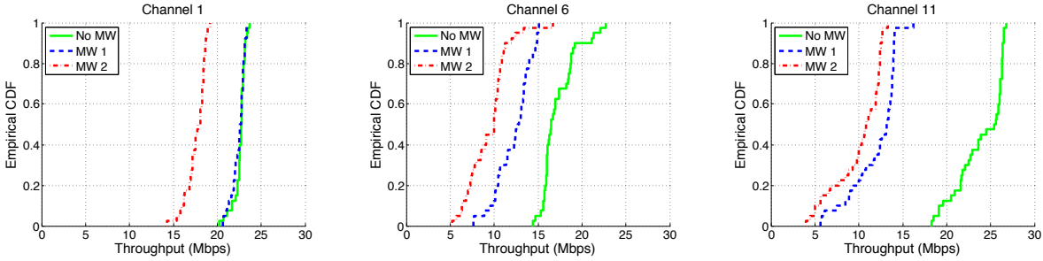
Figure 4. Throughput comparison across 802.11b/g channels 1, 6, 11. The impact of microwave interference is substantially less on channel 1.
